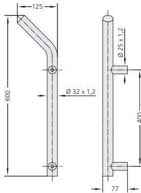
Type ER-32.K
