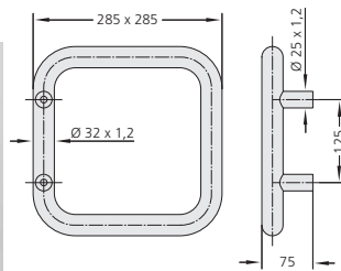
Type ER-32.E
