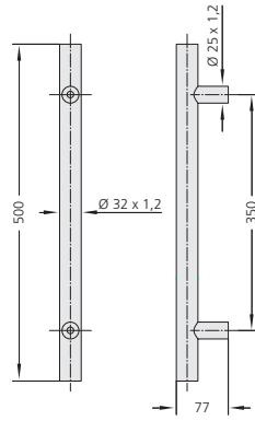
Type ER-32.G
