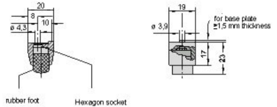
Leg without Lift Lever
