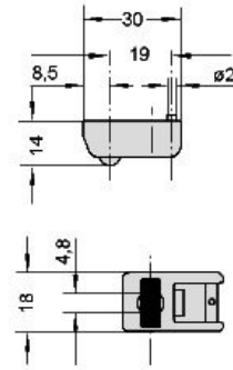
Leg without lift lever
