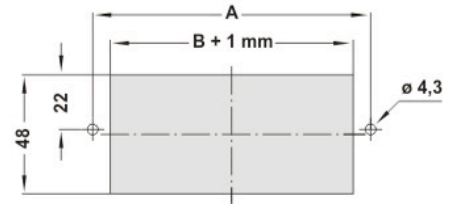
Mounting cutout
